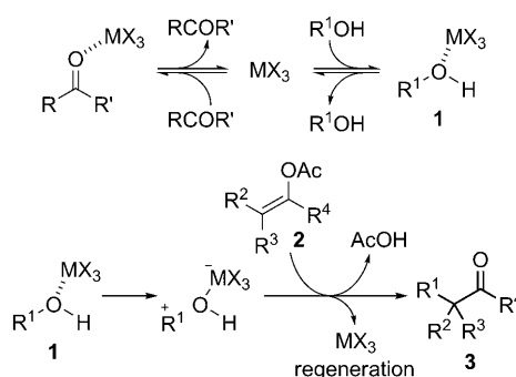
Scheme 1. Proposed reaction mechanism.
